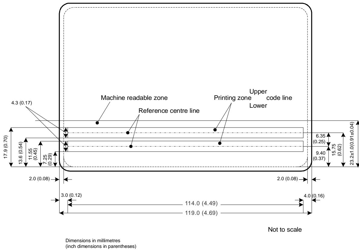
Figure 3. Schematic diagram of the Machine Readable Zone of an MRV-A
